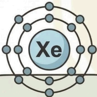
xenon element
